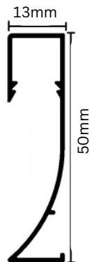
Plug (Left/Right)
