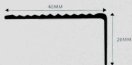
Stair Nosing / L Profile (AL4020)
